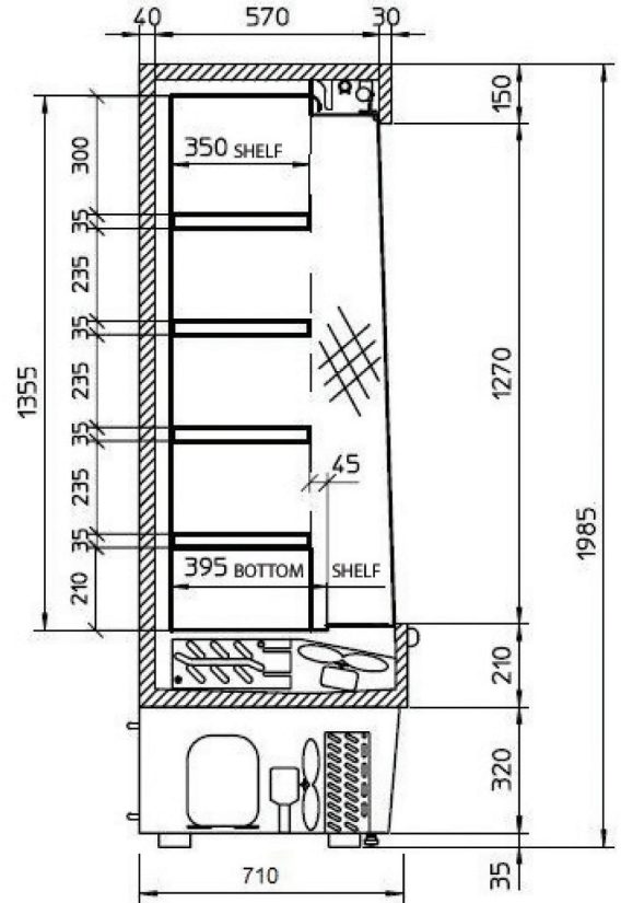
Technical Drawing
